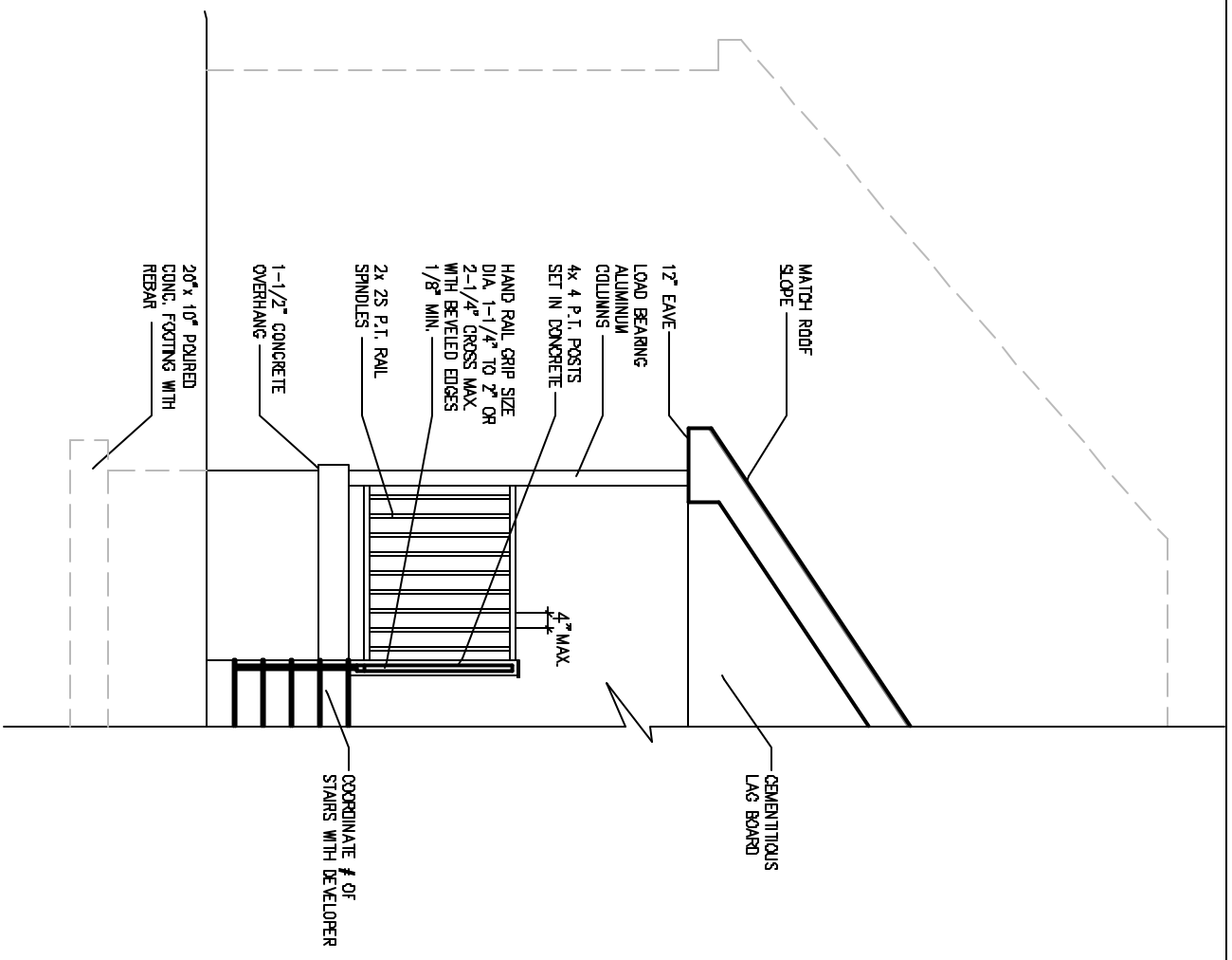
1 A.7 RAISED PORCH SLAB SCALE: 1/4" = 1'-0"
