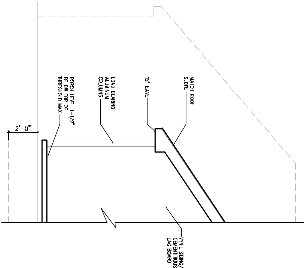
2 A.7 @ GRADE PORCH SLAB SCALE: 1/4" = 1'-0"
