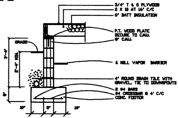
TYP. FOOTER DETAIL SCALE: 3/8" = 1'-0"
